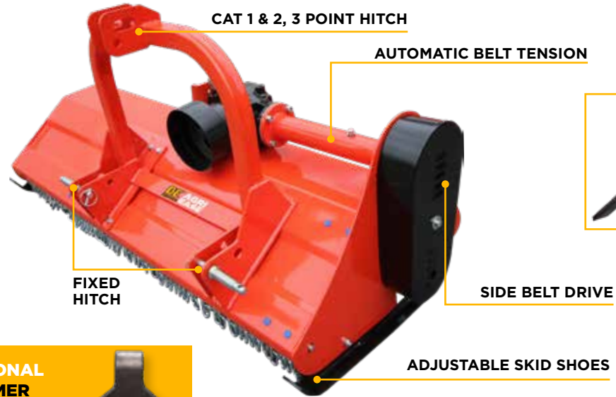
FLAIL
